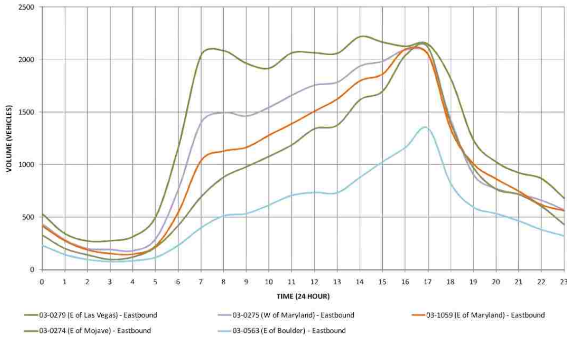
Graph 10: Sahara Avenue – Directional Distribution of Traffic (Eastbound – East of Las Vegas Boulevard) BEFORE
